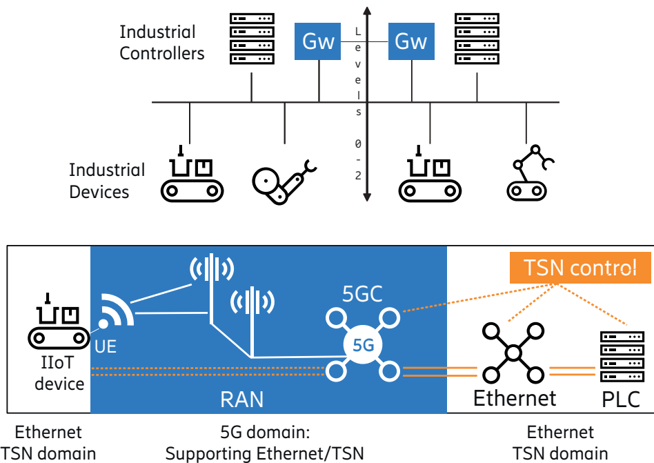
Figure 3: 5G NR will need to support Ethernet-based transport for TSN and industrial controllers
